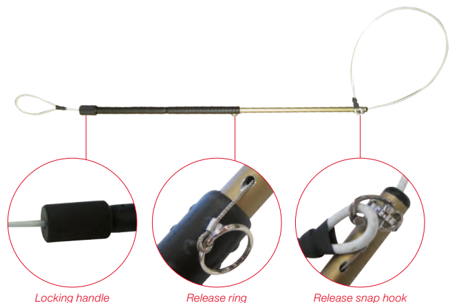
Locking handle
