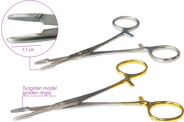
Integrated scissors
