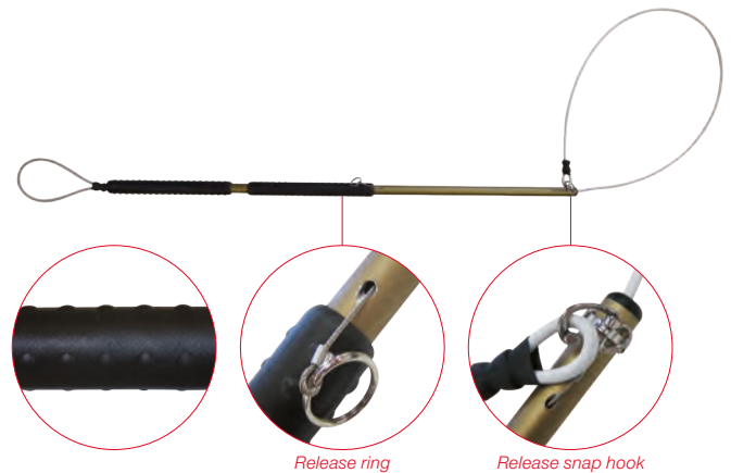
Release ring
