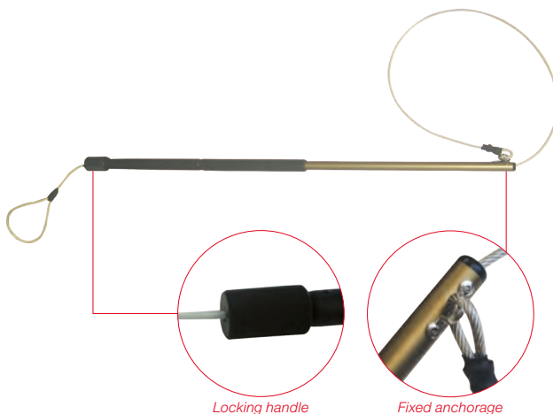
Locking handle
